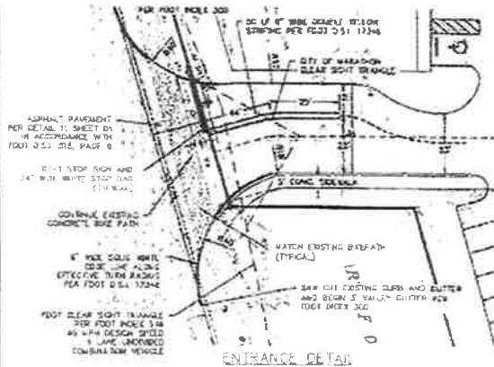
ENTRANCE DETAIL
